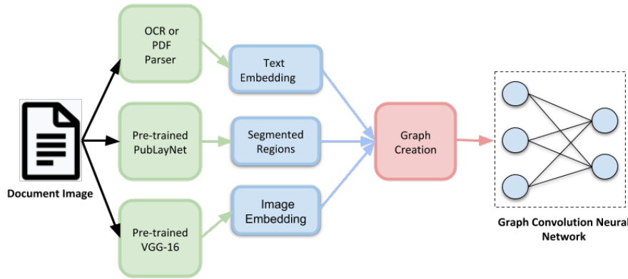
Figure 1: Eff-GNN Framework overview: textual embedding, segmented regions and image embeddings of an image are integrated when the graph of document is formed. Created graph is fed into the Graph Convolution Neural Network for graph classification as document image classification.
